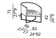
poltroncina - small armchair LOLYTA
