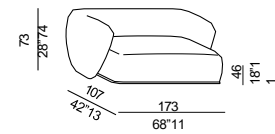
sofa 170
